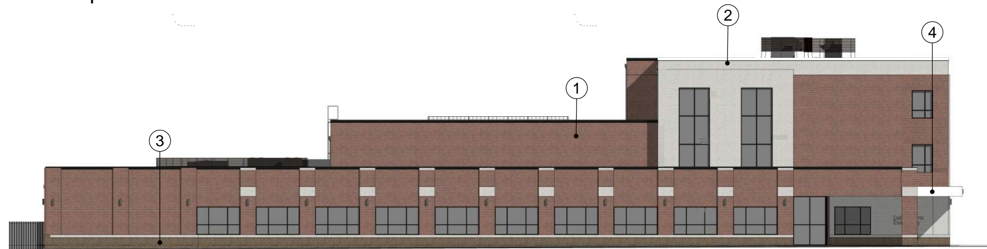
2 NORTH ELEVATION (EAST HAYSTACK STREET)
